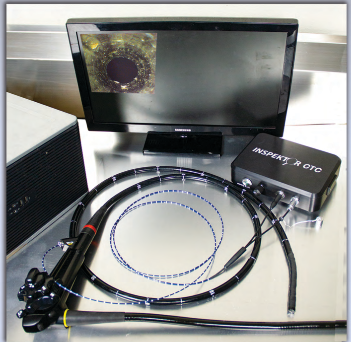
1.8 meter Digital Borescope
